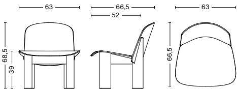
CHISEL LOUNGE CHAIR Width 63 cm Depth 66,5 cm Height 68,5 cm Seat height 39 cm Seat depth 52 cm Weight 9,5 kg
