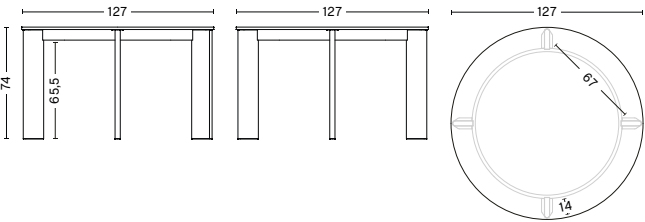
CHISEL 25 TABLE | 4 LEGS Diameter 127 cm Height 74 cm Weight 29 kg
