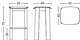
CHISEL 30 BAR STOOL | HIGH Width 42 cm Depth 40 cm Height 75 cm Seat height 75 cm Seat depth 40 cm Weight 8 kg
