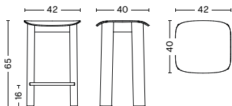
CHISEL 30 BAR STOOL | LOW Width 42 cm Depth 40 cm Height 65 cm Seat height 65 cm Seat depth 40 cm Weight 7,5 kg
