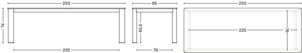
CHISEL 30 TABLE Length 250 cm Width 95 cm Height 74 cm Weight 65 kg
