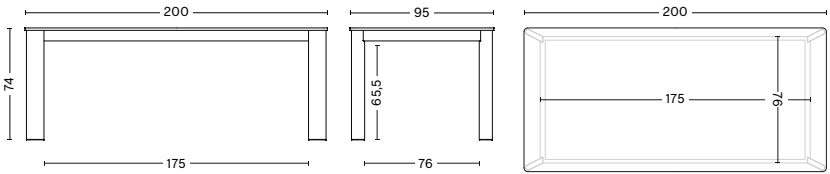
CHISEL 30 TABLE Length 200 cm Width 95 cm Height 74 cm Weight 55 kg
