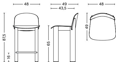
CHISEL 35 BAR STOOL W. BACKREST | LOW Width 48 cm Depth 49 cm Height 87,5 cm Seat height 65 cm Seat depth 43,5 cm Weight 9 kg
