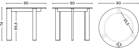
CHISEL 20 TABLE | 3 LEGS Diameter 90 cm Height 74 cm Weight 20 kg
