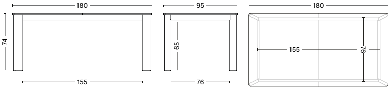
CHISEL 630 TABLE Length 180/280 cm Width 95 cm Height 74 cm Weight 87 kg
