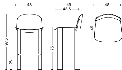
CHISEL 35 BAR STOOL W. BACKREST | HIGH Width 48 cm Depth 49 cm Height 97,5 cm Seat height 75 cm Seat depth 43,5 cm Weight 9,5 kg
