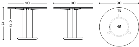
CHISEL 29 TABLE | COLUMN Diameter 90 cm Height 74 cm Weight 40 kg
