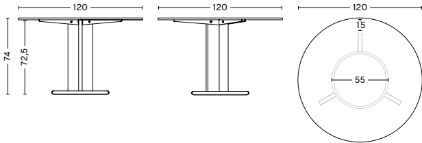
CHISEL 29 TABLE | COLUMN Diameter 120 cm Height 74 cm Weight 50 kg
